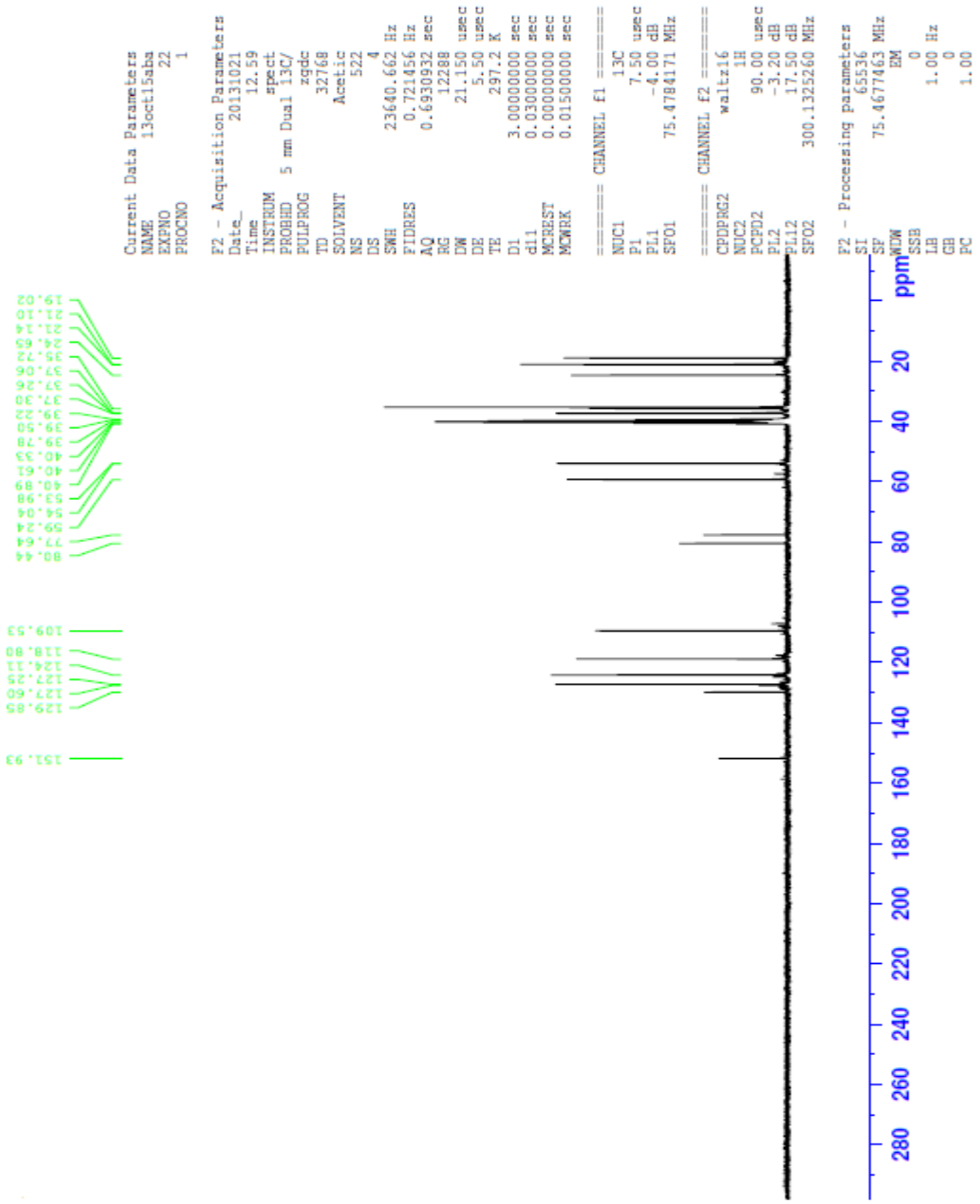
Figure 39: ^{13}\text{C} -NMR spectrum of (AZ-2).
